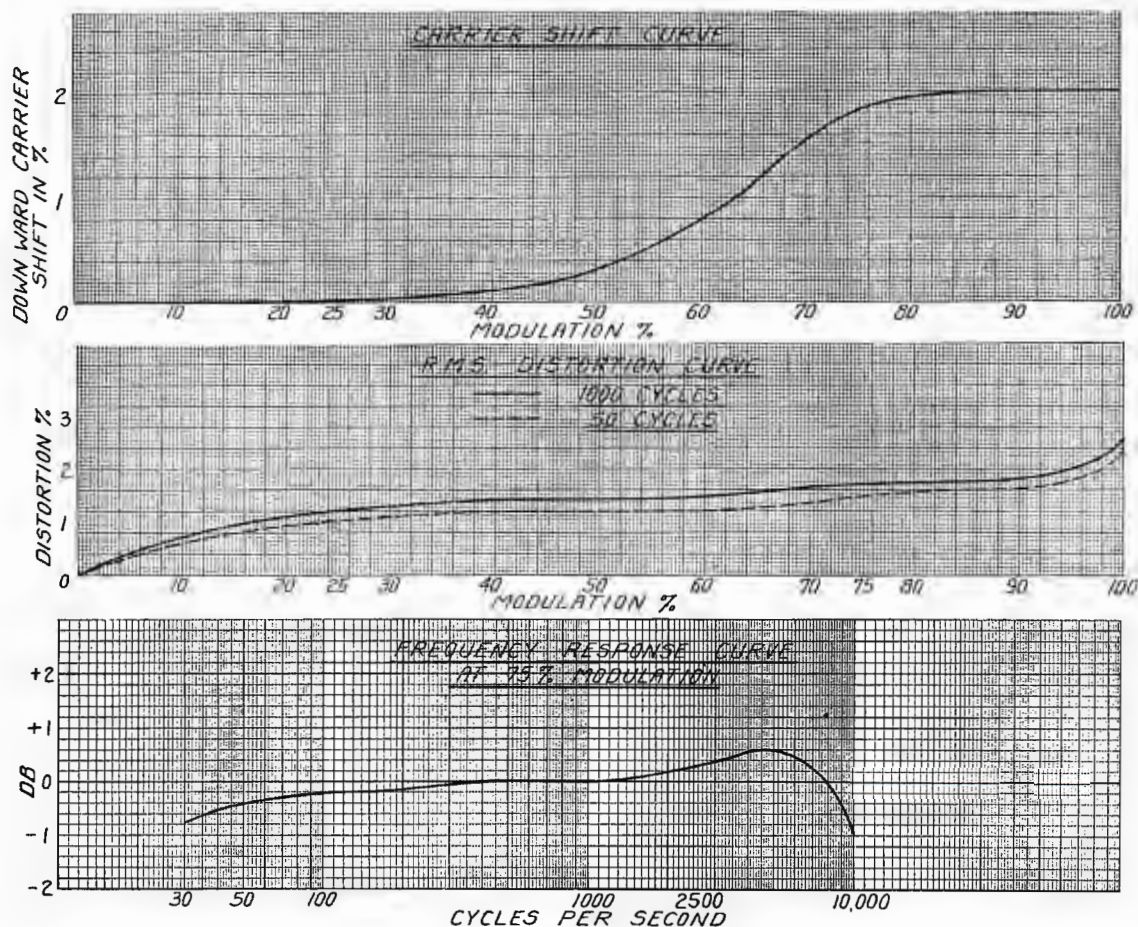
Typical BC-1F Transmitter Characteristics
