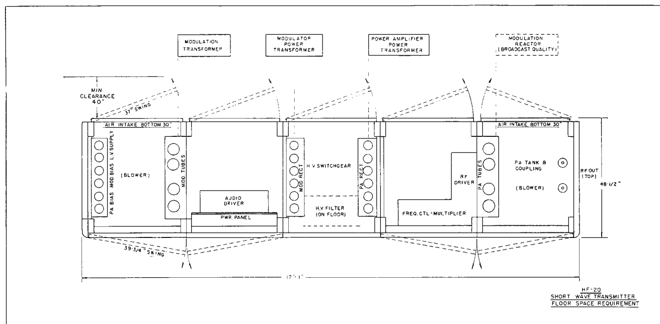
Floor plan of Gates 20 kw short wave broadcast transmitter. Space requirements are considered minimum for a transmitter of this power requirement. External components may be mounted outside of building, where desired.
