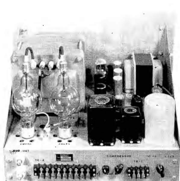
Left, below, is complete radio frequency chassis of CMW-1 transmitter. Right, below, is the speech amplifier-modulator unit with self-contained limiter and 3000 cycle cutoff filter.
