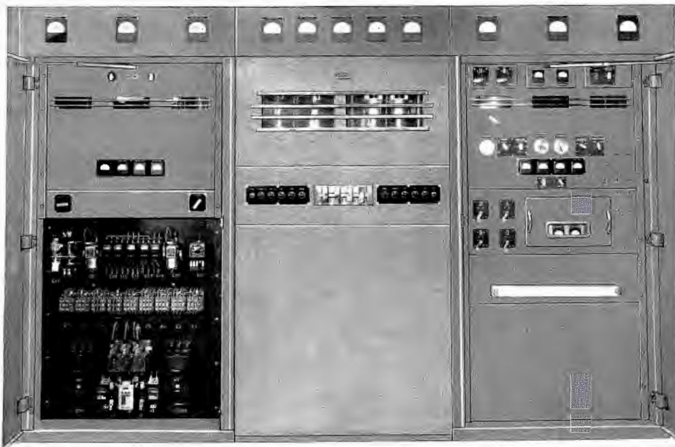
Front of Gates HF-5 and HF-10 transmitters with doors removed. Note massive relay protection to left. Transmitter is in three cubicles which bolt together. Wiring between cubicles is by jumpers between terminal boards, and time consuming "on location" cabling is eliminated.
