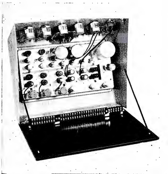
The above illustrates the tilt-back arrangement of the Studioette cabinet for reaching tubes, attenuators, and terminal connections instantly. For reaching under-chassis parts, the top of the cabinet is removable, making complete instantaneous 100% accessibility possible.
