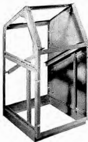
Above, basic section with top, back cover, and front panel removed. Electrical shield is mounted on right side, and is used as needed.
