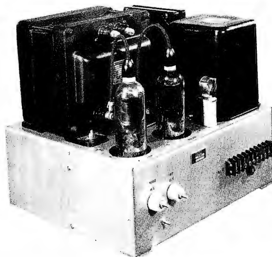
Above, left, the low voltage power supply deck. Right, the main high voltage supply delivering 2300 volts to power amplifiers and modulators.
