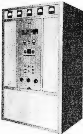
For heavy duty service, the Gates 1000 - watt amplifier stands 78" high, 40" wide and 36" deep. Operates from 220 volts single phase.
