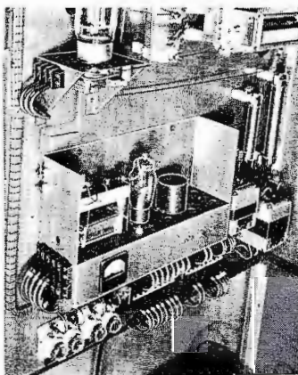
Oscillator unit holds two crystals and ovens and may be removed almost instantly for under chassis servicing.
