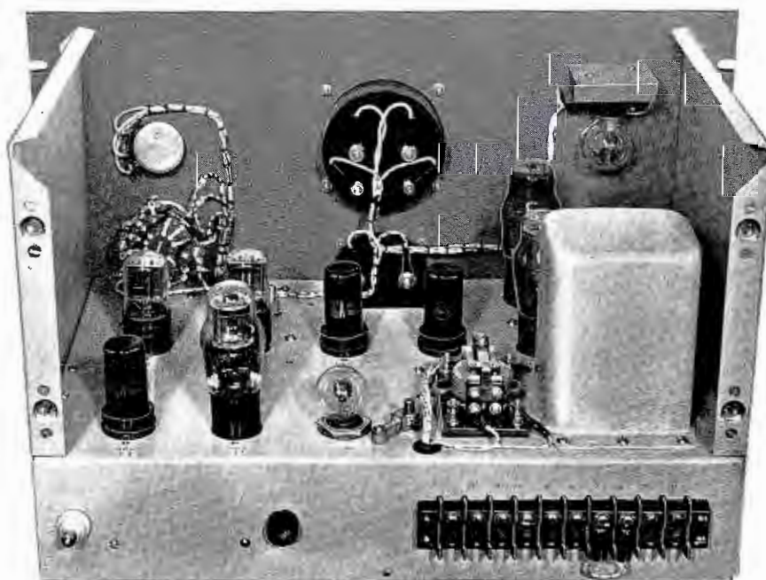
Rear dust cover removed—MO-2639 Modulation Monitor
