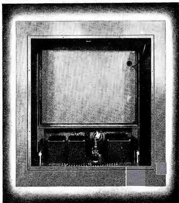
Rear view of the BF-E-10 transmitter shows the power supply in the bottom and the transmitter portion just above. The inside cover over the transmitter chassis is easily taken off by removing the four thumb screws in the corners and disconnecting the coaxial output feed line at the fitting on top of the transmitter.
