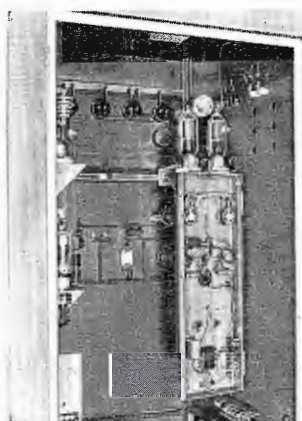
Swing out audio deck shows portion of 100% accessibility of all parts. Every part in the BC-500GY transmitter can be reached in a matter of seconds.
