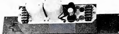
Figure D—Back view of SA-72 rack mount preamplifier. Note the shock mounting of tubes, test jacks for plate current, metering and isolation of input and output terminations.
