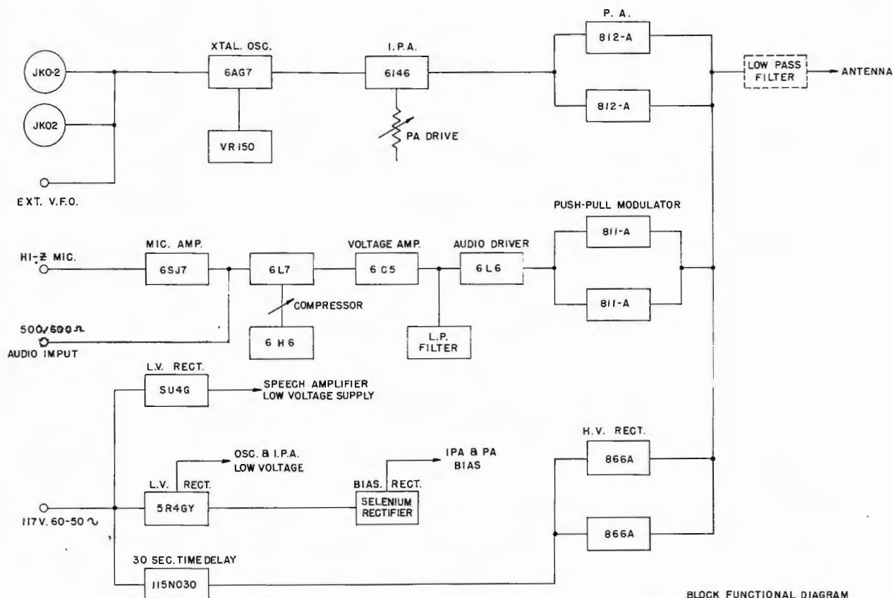
BLOCK FUNCTIONAL DIAGRAM 250 W. COMMUNICATIONS TRANSMITTER CMG1-M4575
