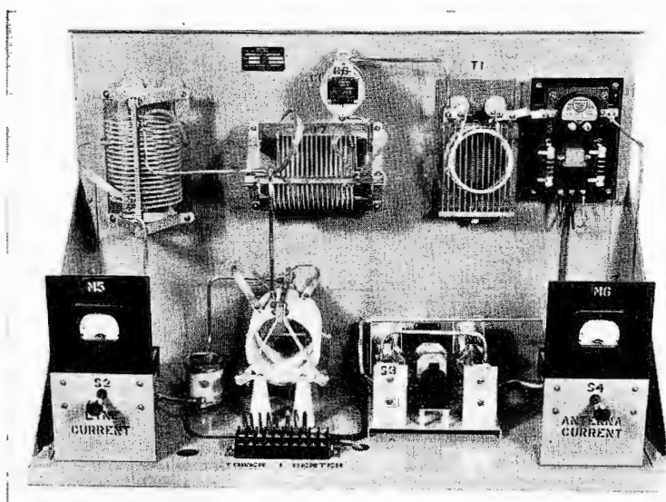
Indoor Shelf Type Coupler
